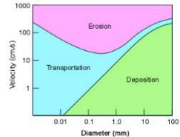
Hjulstrom's Diagram http://www.columbia.edu/~vjd1/streams_basic.htm
